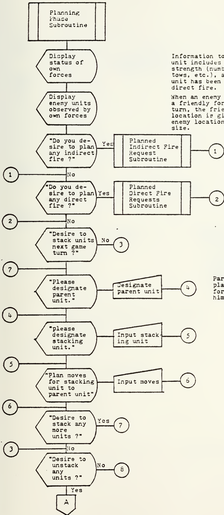
FIGURE VII.7 FLOWCHART OF PLANNING PHASE SUBROUTINE
